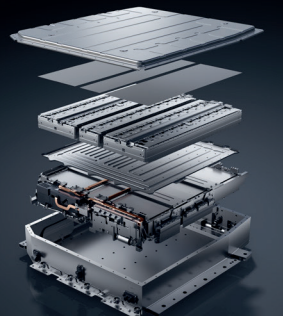
CATL-developed Off-road Dedicated Battery
